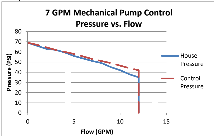
Figure 2 - Bubble-Up® Interactive™ Outlet Flow vs. Pressure 7 GPM
