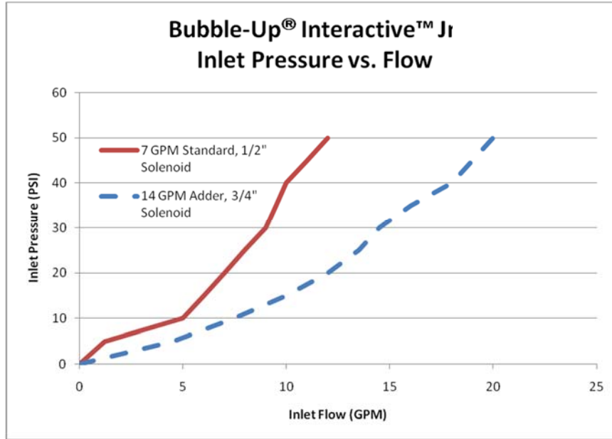
Figure 1 - Bubble-Up® Interactive™ Inlet Pressure vs. Flow
